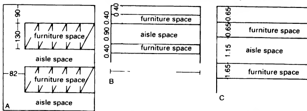
⑪ Circulation/furniture areas for various filing systems
